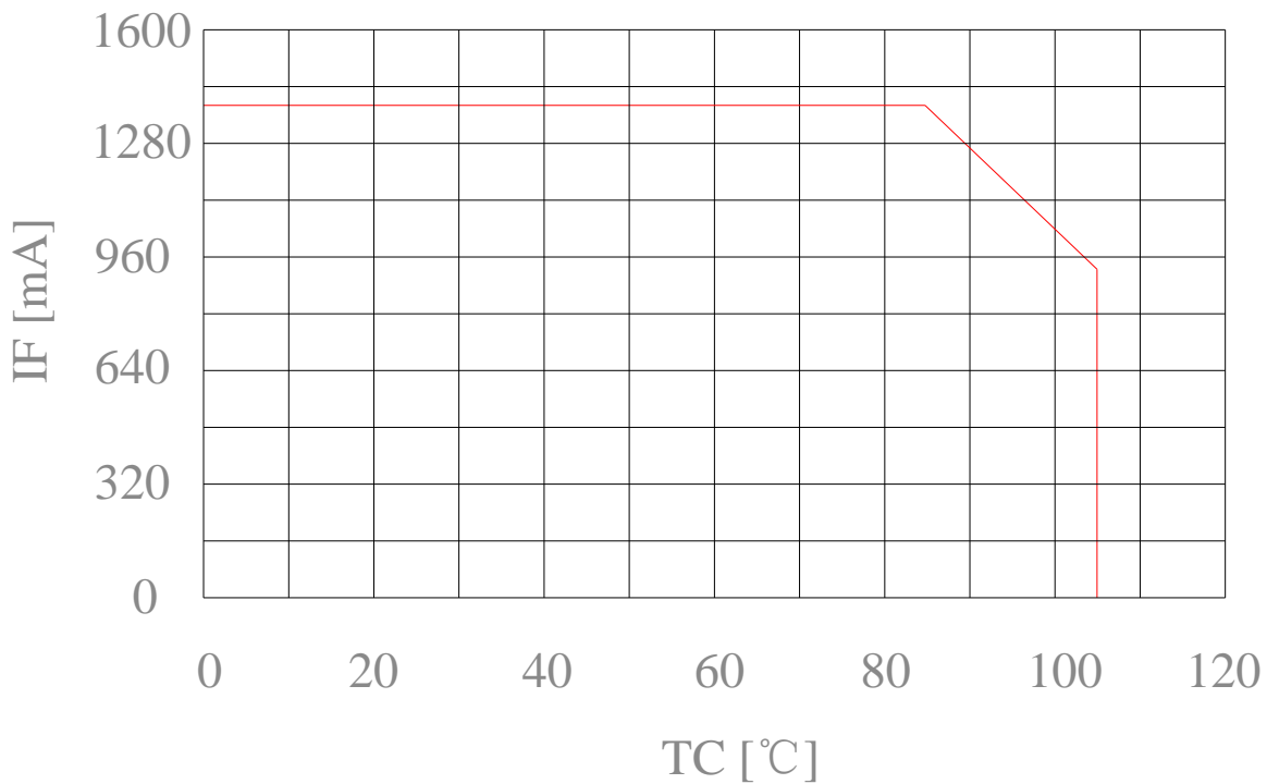
Case Temperature VS. Allowable Forward Current
